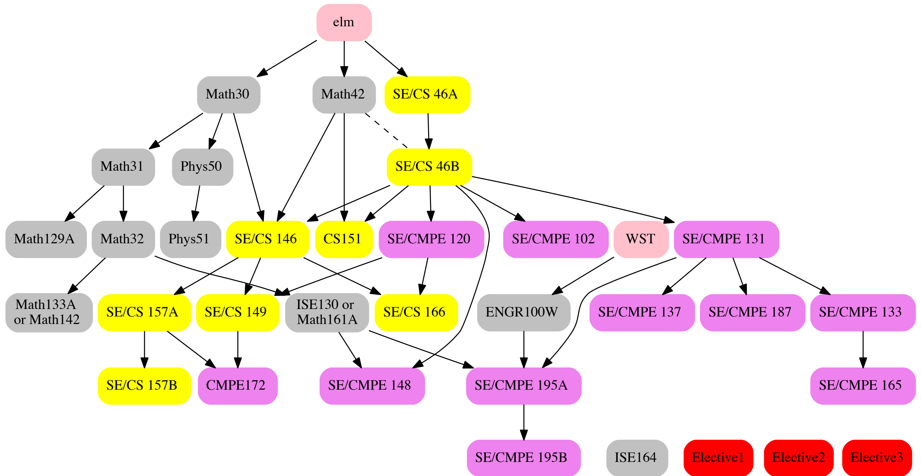
Prerequisite relationships for the BS SE degree, 2012-2014 catalog.
